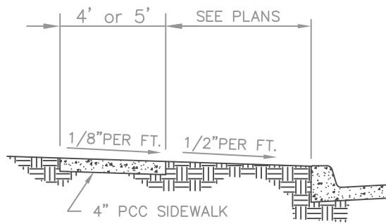
TYPICAL SIDEWALK SECTION
