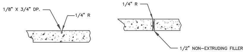
CONTRACTION JOINT
