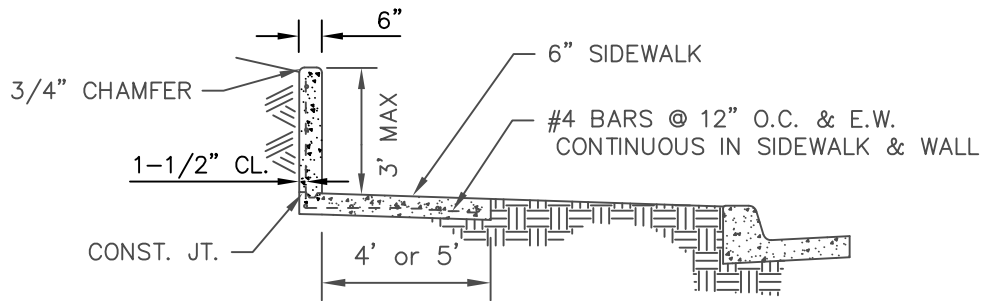
SIDEWALK WITH INTEGRAL RETAINING WALL
